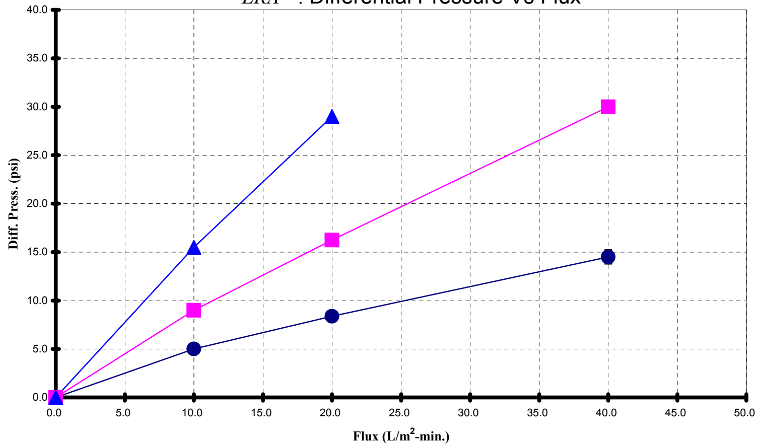
Figure 3 LRA ® : Differential Pressure Vs Flux
